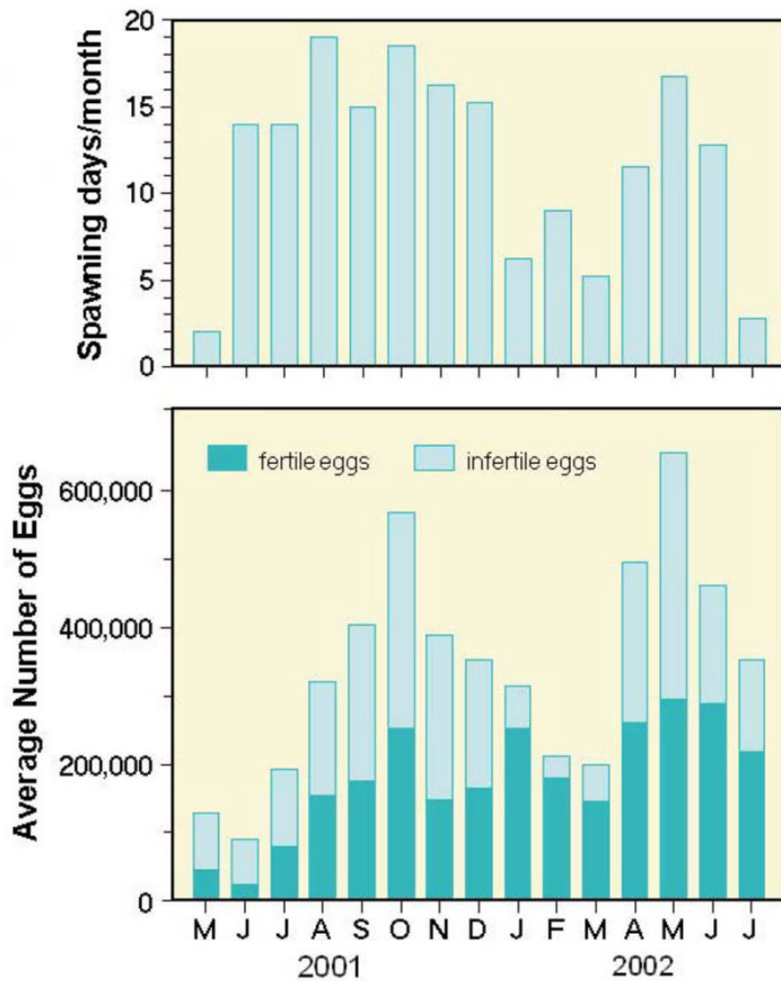
Fig. 2: Spawn frequency and egg production of captive-reared amberjack broodstock in outdoor spawning tanks.
