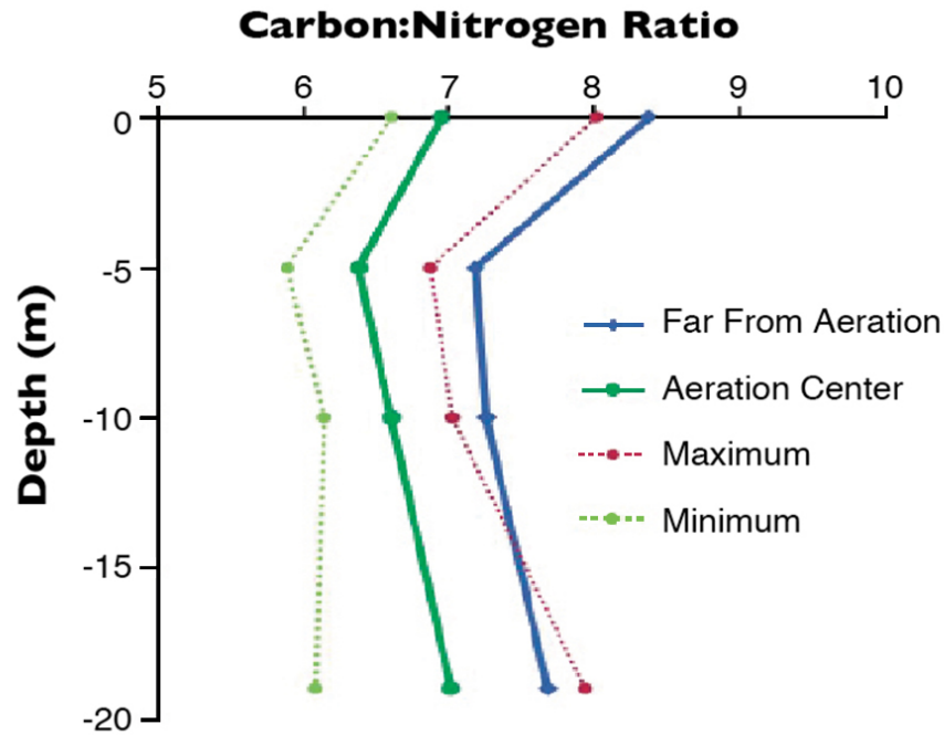
Fig. 2: Mean carbon: nitrogen ratios for suspended particulate organic matter at two locations. Maximum and minimum values at the aeration center are also shown.
