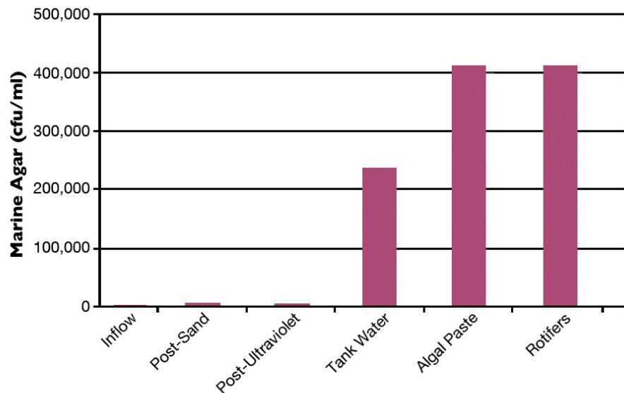
Fig. 2: Changes in cultivable bacteria levels through each step of water treatment. Initial hatchery design included sand filtration, 50- and 5- \mu m cartridge filtration and ultraviolet sterilization. The improved hatchery design included vacuum degassing, glass filtration, 5- and 1- \mu m cartridge filtration and U.V. sterilization.
