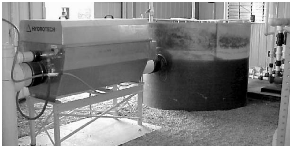
Drum filter (left) for solids removal from a recirculating system.
