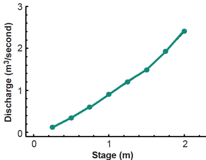
Fig. 1: A rating curve can determine channel or stream flows.
