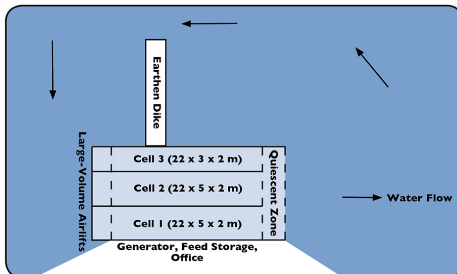
Diagram of the Wujiang farm IPA system.
