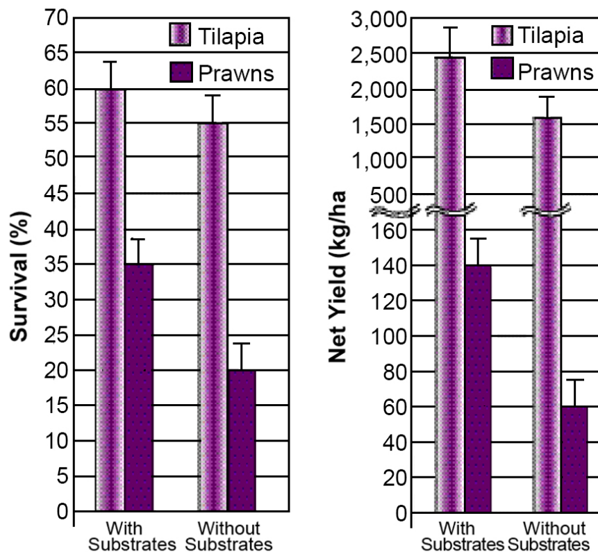
Fig. 1: Survival of tilapia and prawns in ponds with and without periphyton substrates. Fig. 2: Net production of tilapia and prawns after 145 days in ponds with and without periphyton substrates.
