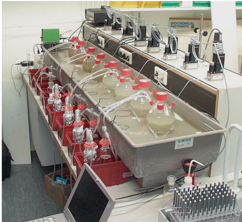
The test setup used eight units with controlled gas flow.
