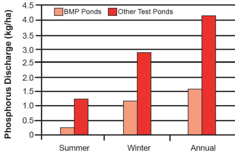
Fig. 2: Summer, winter, and average annual mass discharge of total phosphorus from study ponds.
